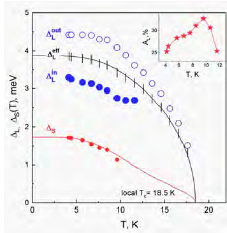
Fig. 1. The obtained temperature dependencies \Delta_L^{\text{in}}(T) , \Delta_L^{\text{out}}(T) , and \Delta_S(T) (rounds) were approximated using functions calculated within the framework of the two-band theoretical model by Moskalenko and Suhl (solid lines) [7, 8], where the effective amplitude of the larger gap is taken as the average: \Delta_L^{\text{eff}} = (\Delta_L^{\text{out}} + \Delta_L^{\text{in}})/2 (vertical strokes). Inserted graph shows anisotropy of the larger SC gap A_L = 100\% \cdot [1 - \Delta_L^{\text{in}}/\Delta_L^{\text{out}}] \approx 30 \pm 5\% .
