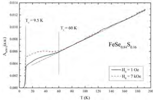
Fig. 1. Temperature dependences of microwave absorption for the FeSe 0.84 S 0.16 sample obtained in a magnetic field of 1 Oe and 7 kOe. The dash-dotted line shows the linear behavior. Vertical lines correspond to the temperatures of superconducting and structural transitions.
