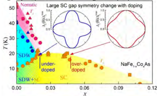
Fig. 1: Electron doping phase diagram of Na(Fe,Co)As pnictides, and a sketched change in the large gap angle distribution in the k -space with doping.
